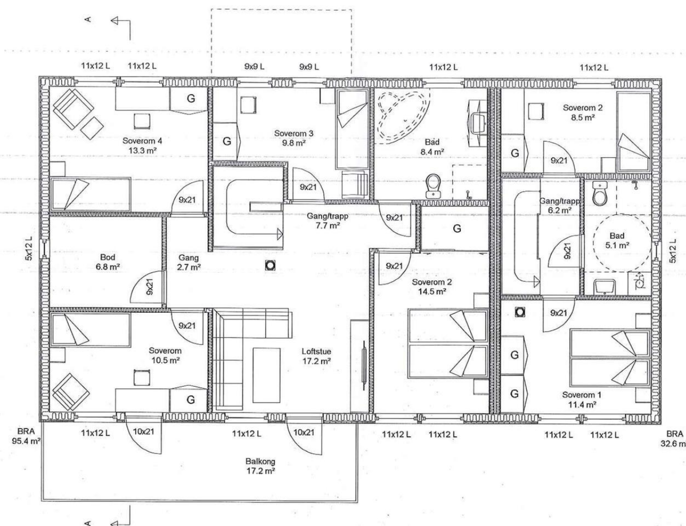
Bileilighet
